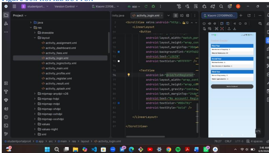
Figure 11.RESULTS BUTTON
