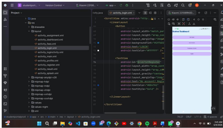
Figure 9. DASHBOARD SCREENS
