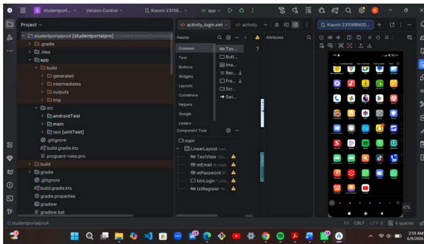
Figure 3.EMULATOR APP
